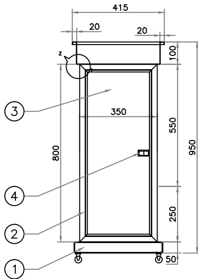
BACK VIEW (OPERATOR SIDE)
