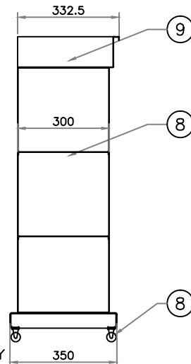
DETAIL X
